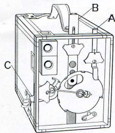
This diagram shows the position of slide B when the smallest stop opening is in front of the lens.
