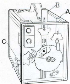
A—Exposure Slide B—Stop Opening Slide C—Exposure Lever
